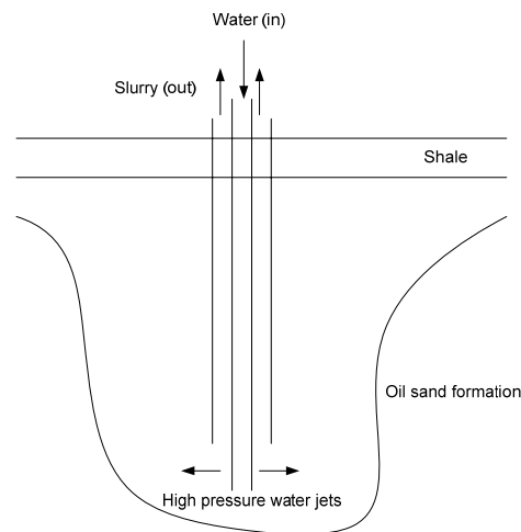
Figure 2-3 Borehole mining schematic
