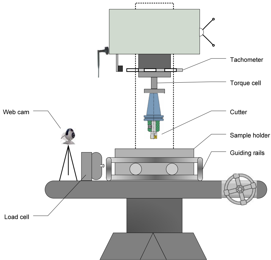
Figure 4-1 Instrumented mill
